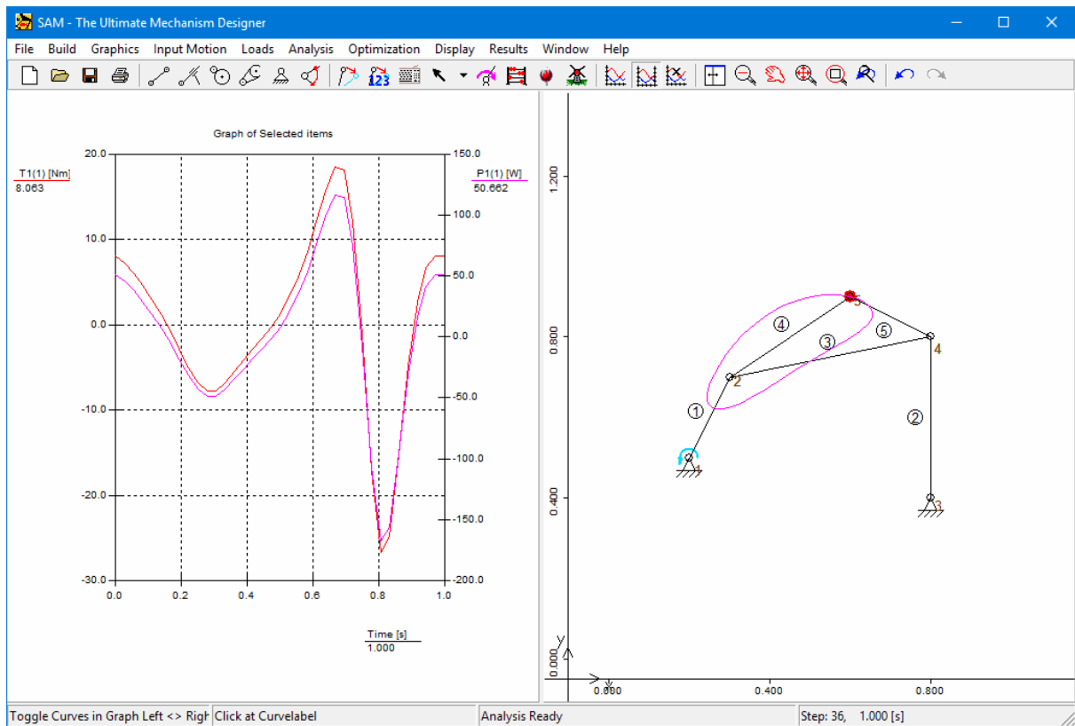
SAM 7.0 results: Torque (left) &amp; Power (right) in element 1 at node 1
