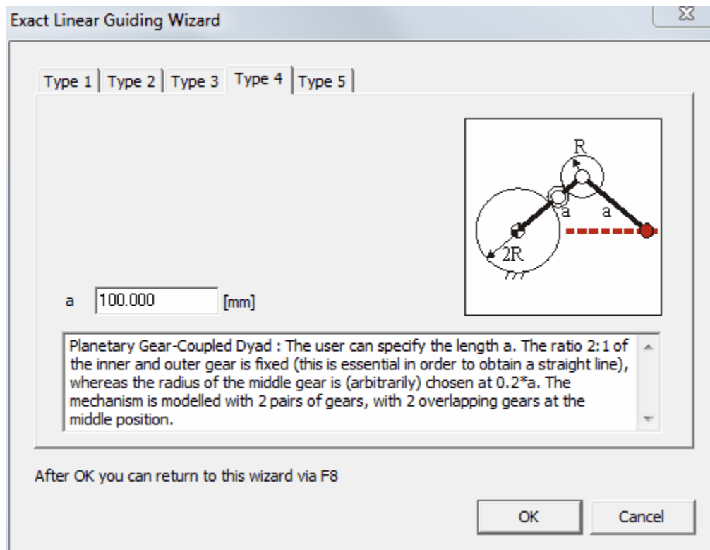
Exact Straight Line Motion Wizard: Planetary Gear-Coupled Dyad
