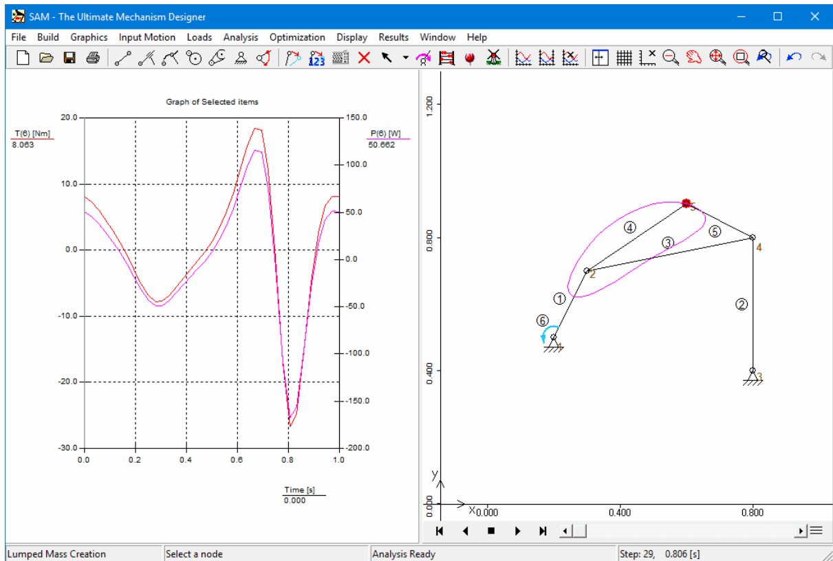
SAM 8.0 results: Torque (left) &amp; Power (right) in element 6 (=motor).
